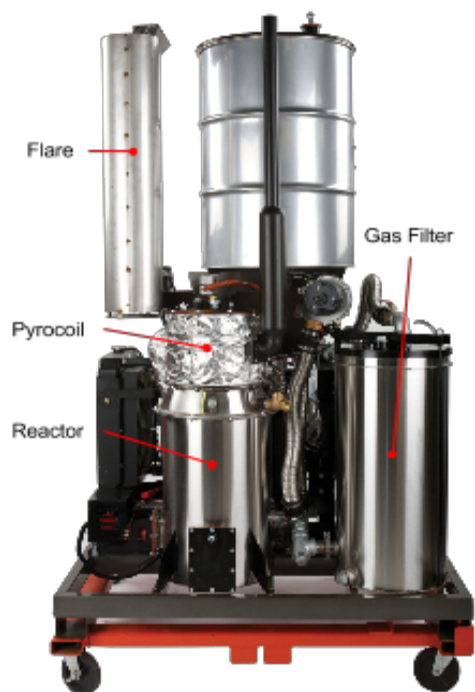
Reactor side of the Power Pallet
